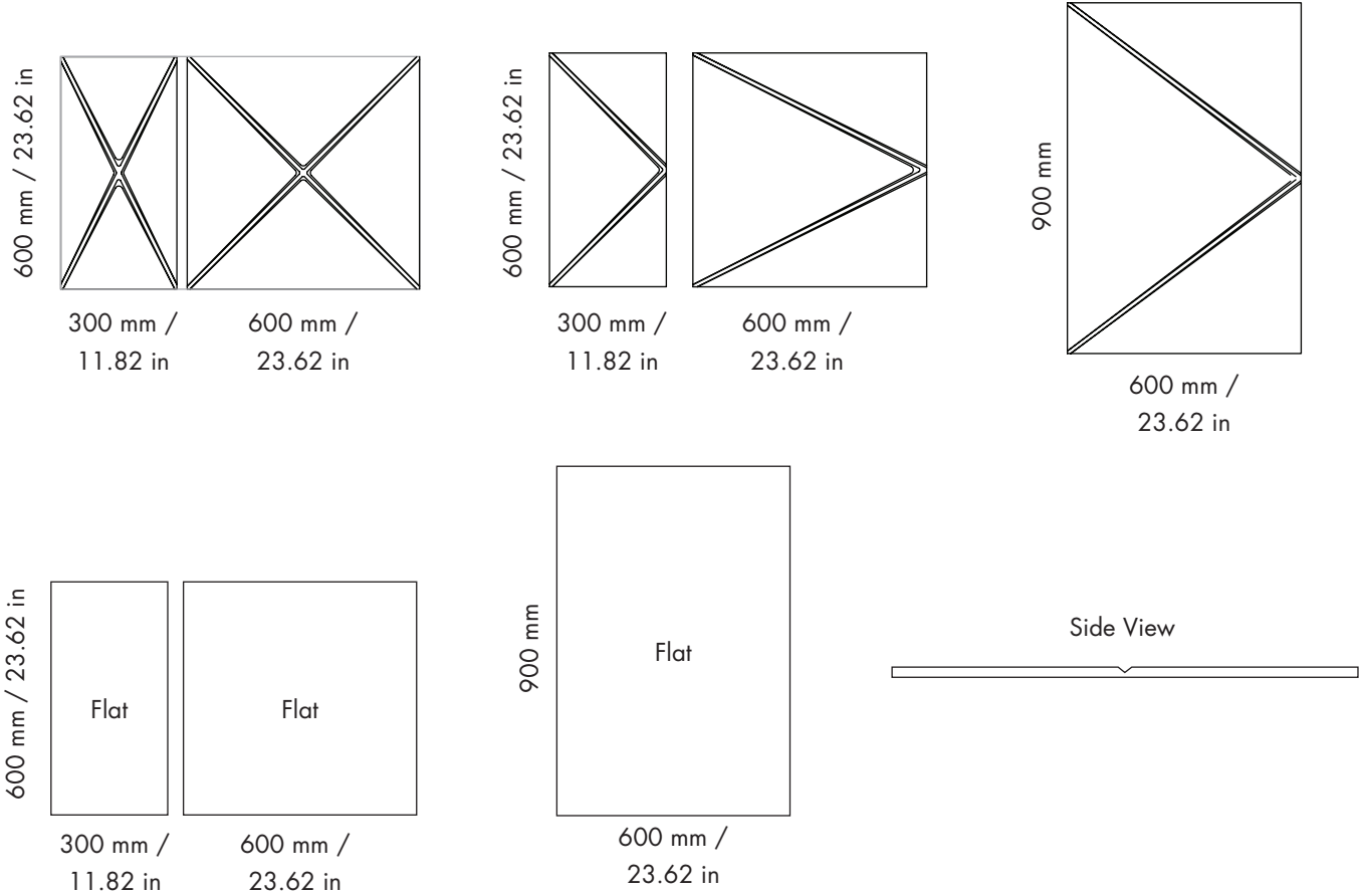
Sample Layout
