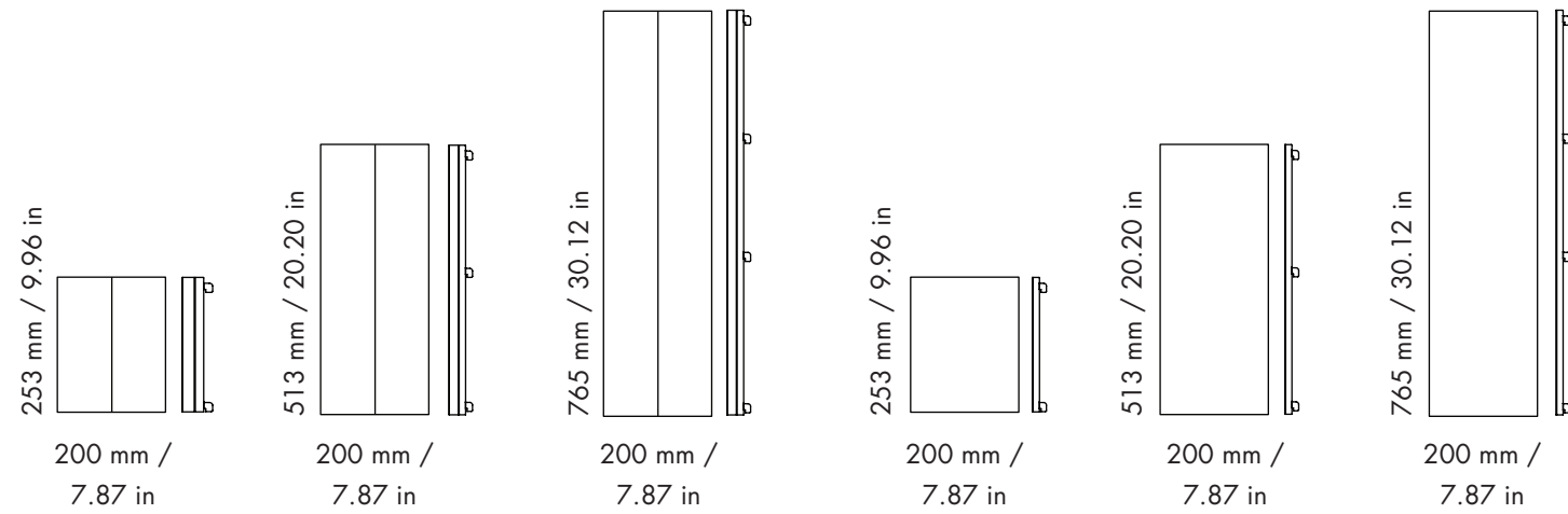
Side Views
