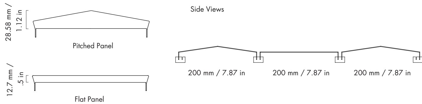
Sample Layout
