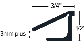
ETR 38 Ceramic Tile to LVT TRANSITIONS FROM 3MM+ LVT TO 3/8" TILE ON MORTAR FINISH: EA, EN, BRZ
