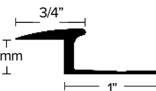
LVT 190 Carpet to LVT TRANSITIONS FROM 9MM LVT TO CARPET. FINISH: EA, EN, BRZ
