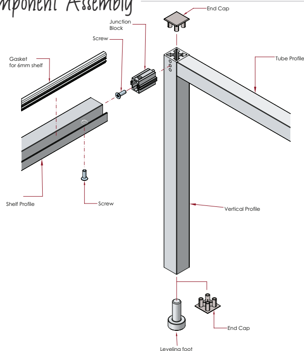
Inset shelves (For use with 6mm shelf material)
