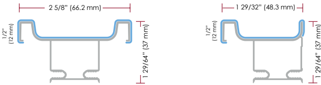
8059 Double Channel 8074 Single Channel
