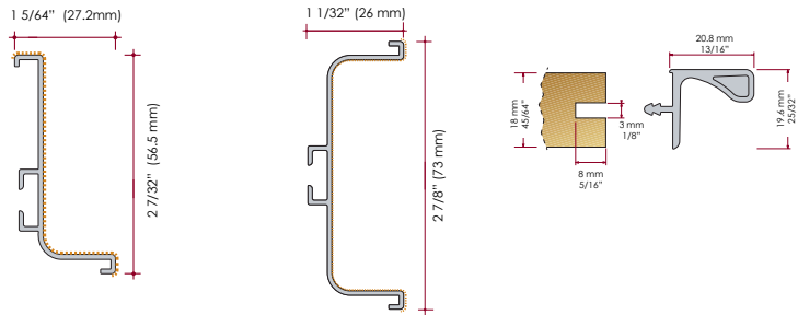
8006 J-Channel 8007 C-Channel 1730 Upper
