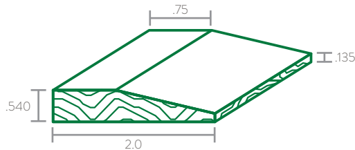
Type "A" Flush Reducer
