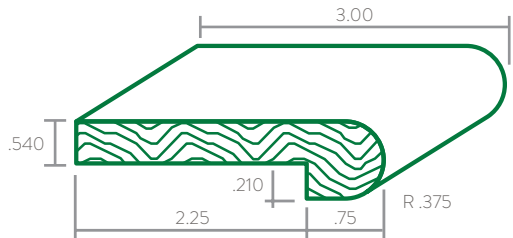
Flush Bullnose Stair Nosing
