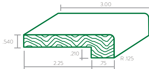
Flush Square Stair Nosing
