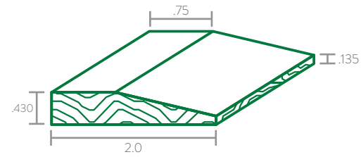
Type "A" Flush Reducer
