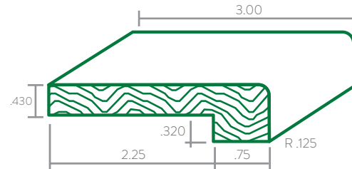
Flush Square Stair Nosing
