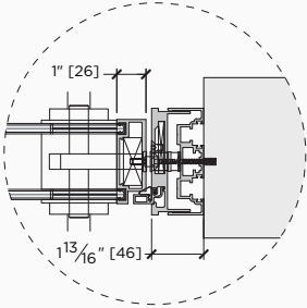
DOOR TO WALL
