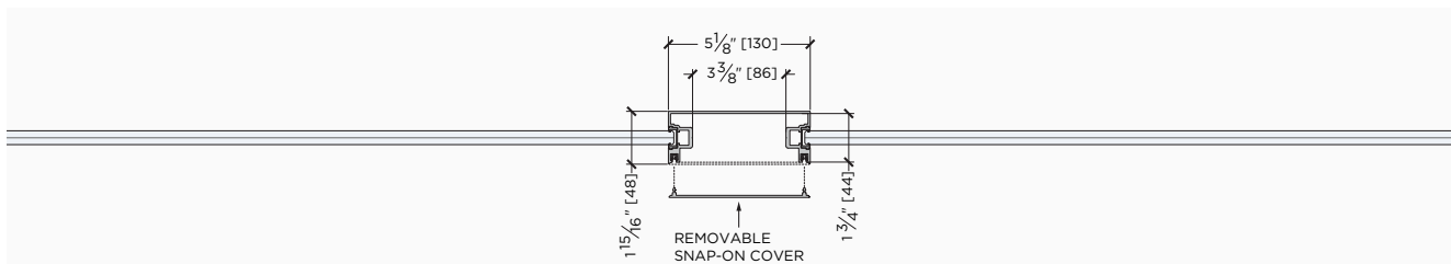
WIRE MANAGEMENT CHASE
