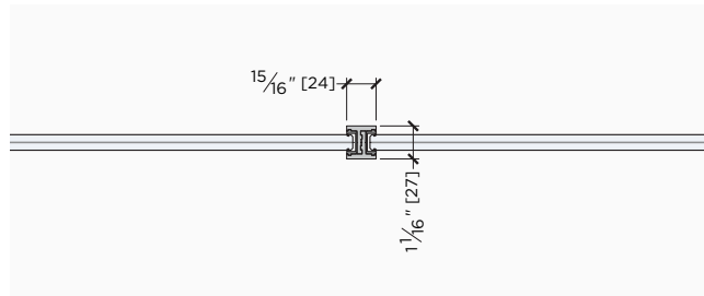
VERTICAL MULLION
