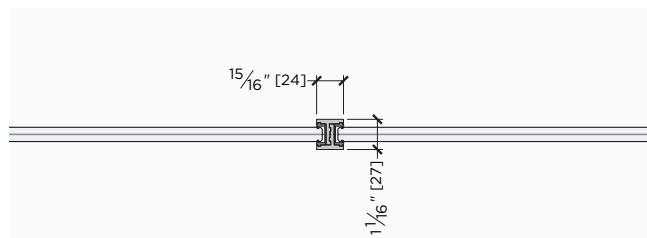
VERTICAL MULLION
