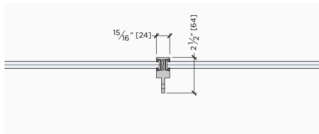
VERTICAL MULLION SHELF SINGLE SIDE
