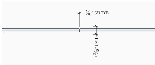
BUTT JOINT
