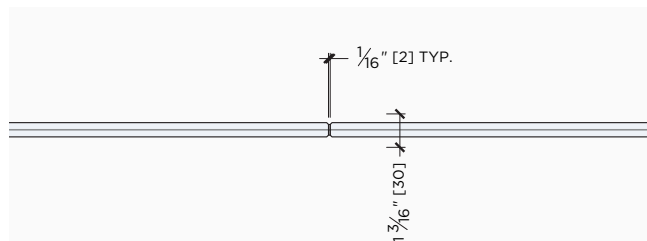
BUTT JOINT
