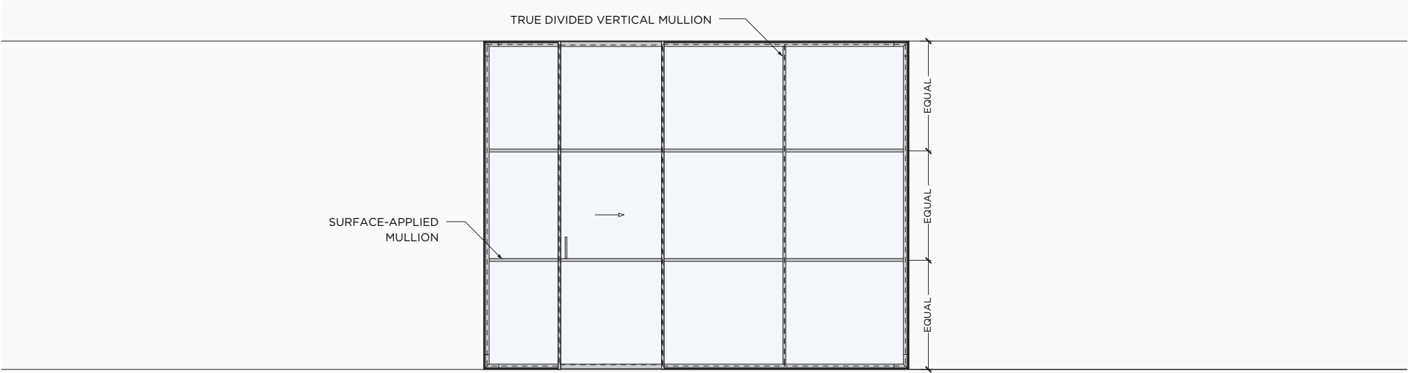
THREE-DIVISION HORIZONTAL MULLIONS (W/ SLIDING DOORS)
