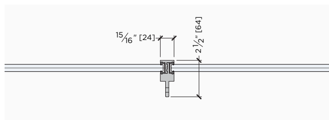
VERTICAL MULLION SHELF SINGLE SIDE
