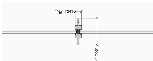
VERTICAL MULLION SHELF DOUBLE SIDE
