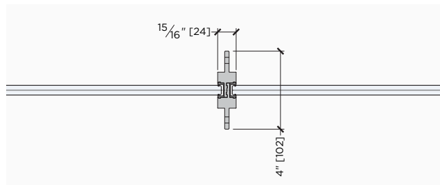
VERTICAL MULLION SHELF DOUBLE SIDE
